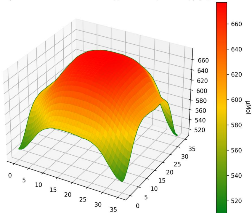
PPFD 3D Heatmap LT-5632 - 6500K - Distance @ 600mm - power supply @ 3500mA
